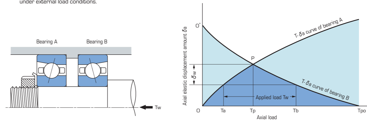
Figure 5.3 Fixed-position Preload
