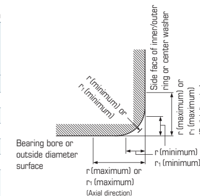
● Table 8.8 Chamfer Dimensions for Radial Bearings (Excluding Tapered Roller Bearings) Unit: mm
